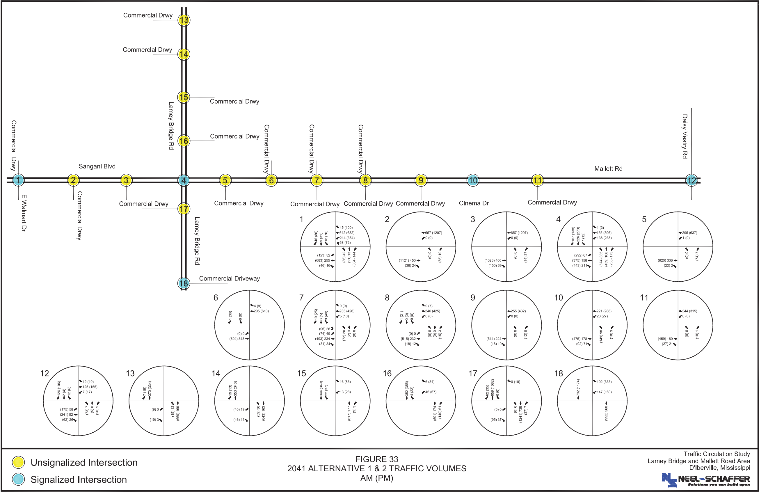
Figure 33. 2041 Alternative 1 & 2 Volume
