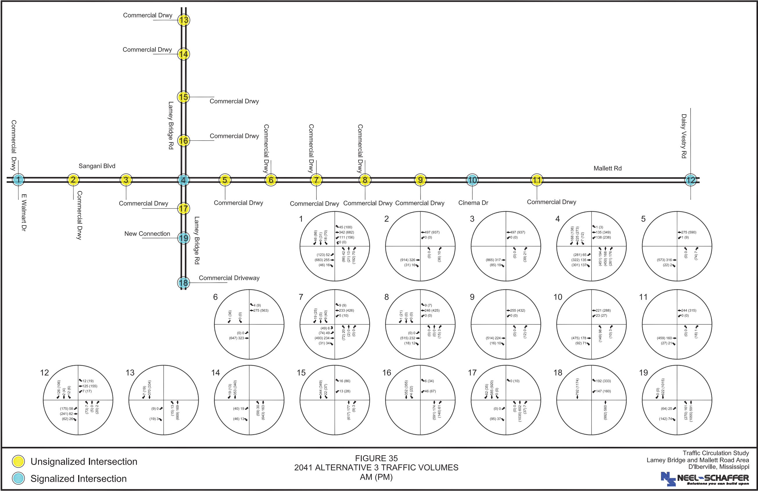
Figure 35. 2041 Alternative 3 Volume
