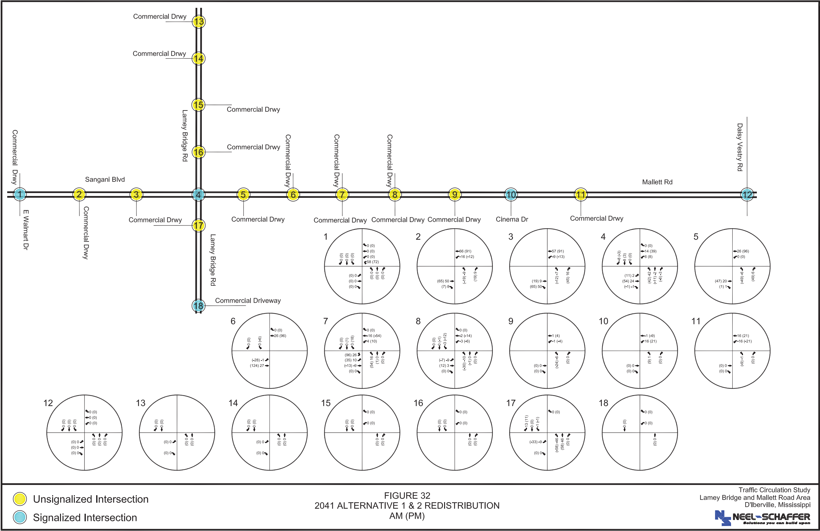
Figure 32. 2041 Alternative 1 & 2 Redistribution
