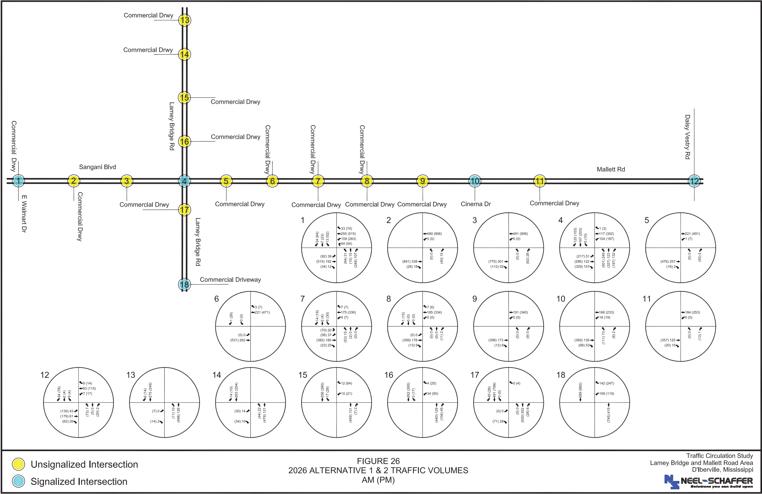
Figure 26. 2026 Alternative 1 & 2 Volume
