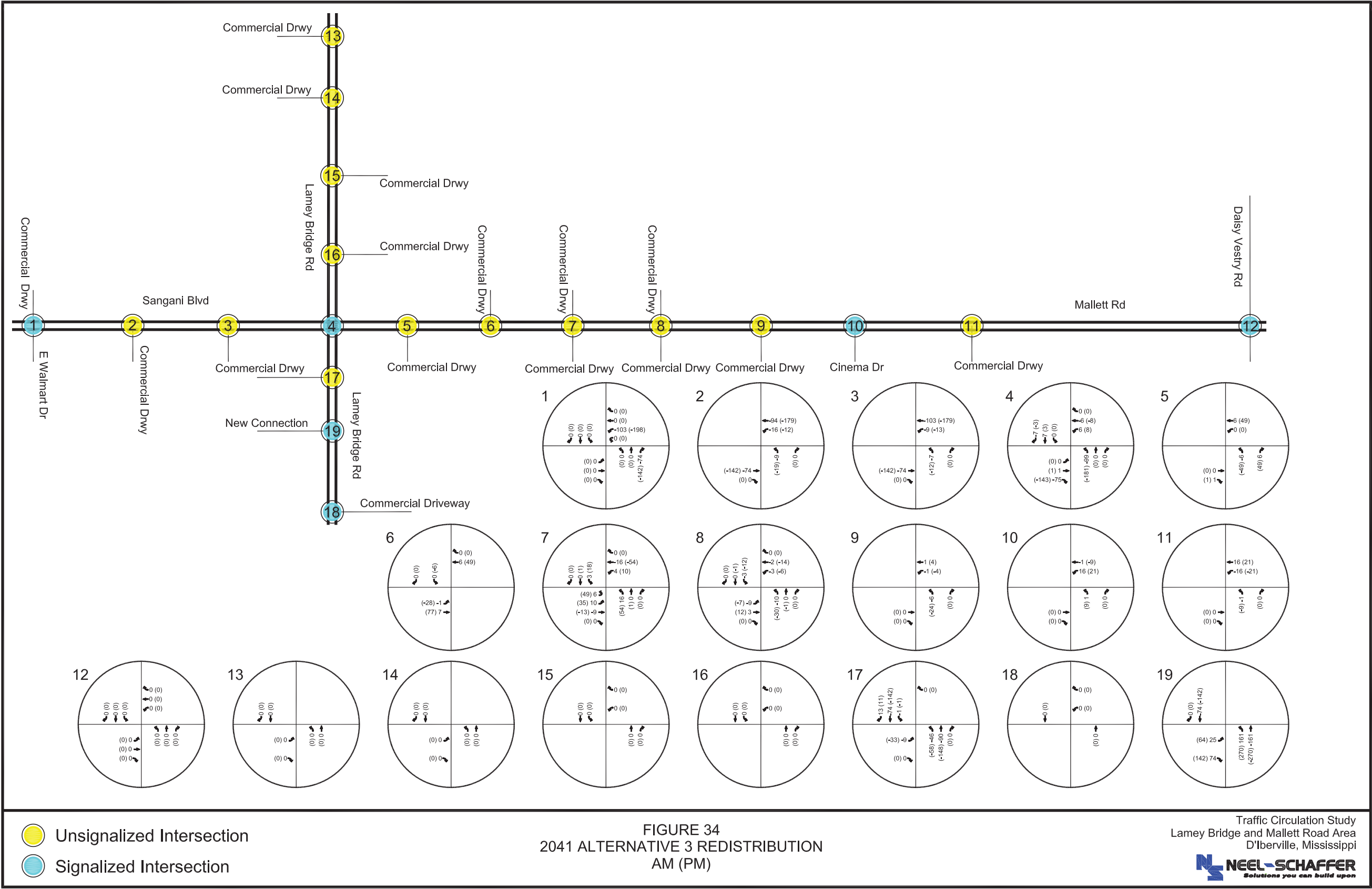
Figure 34. 2041 Alternative 3 Redistribution
