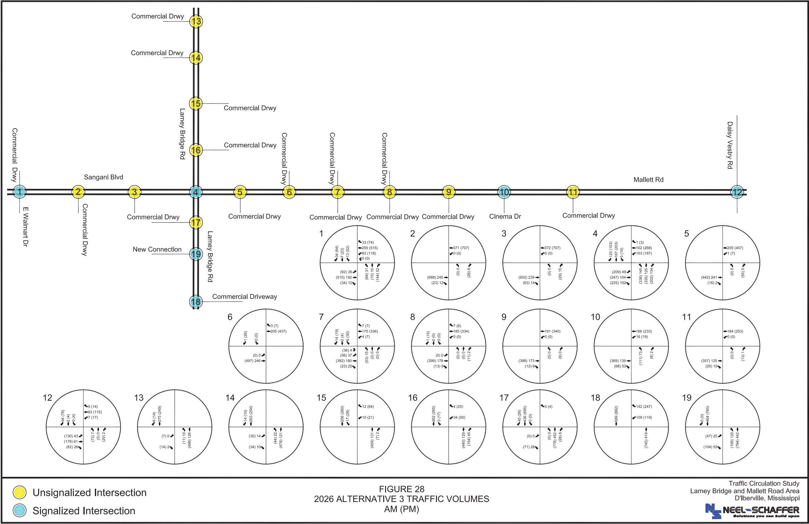
Figure 28. 2026 Alternative 3 Volume
