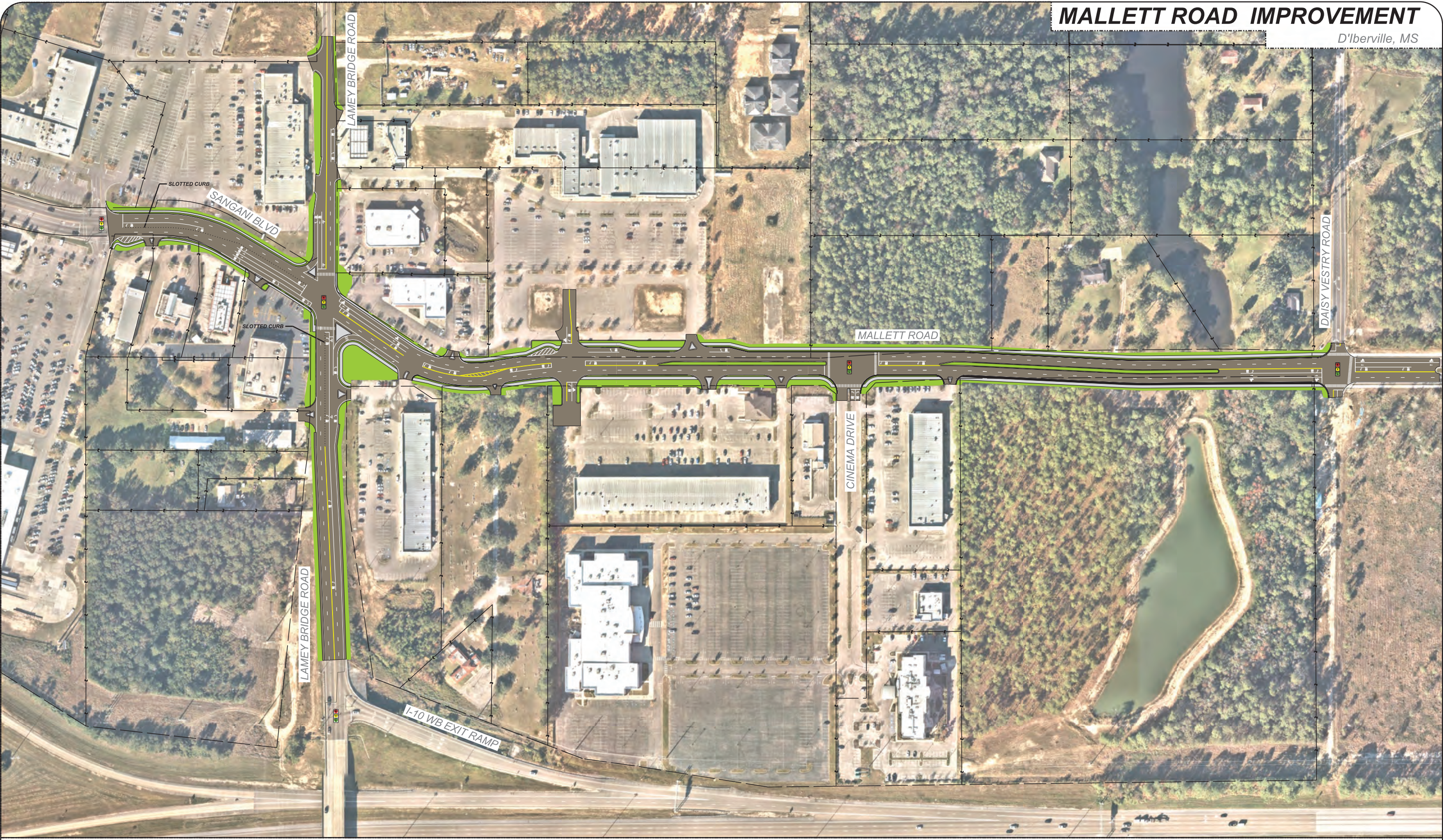
Figure 22. Alternative 2 Layout
